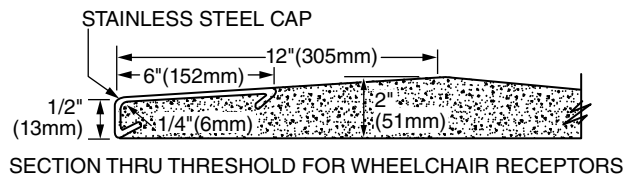
SECTION THRU THRESHOLD FOR WHEELCHAIR RECEPTORS
