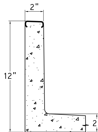
SECTION 4 SHOULDER W/ ST/ST CAP
