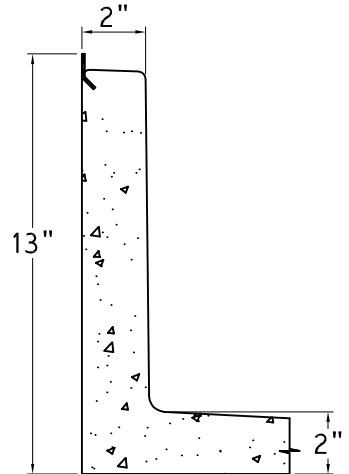
SECTION 5 SHOULDER W/ FLANGE
