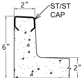
SECTION 2
